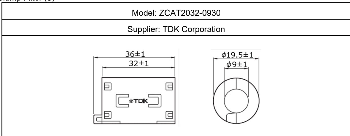
Clamp Filter (5)
