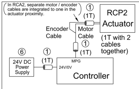
Controller : PCON-CA/CB/CGBCFA/CFB/ CGFB/CBP/CGBP/CYB/ PLB/POB/PSEP-C/CW
