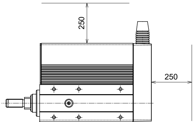
j) RCP2-SRA4R (Same for other short type actuators)
