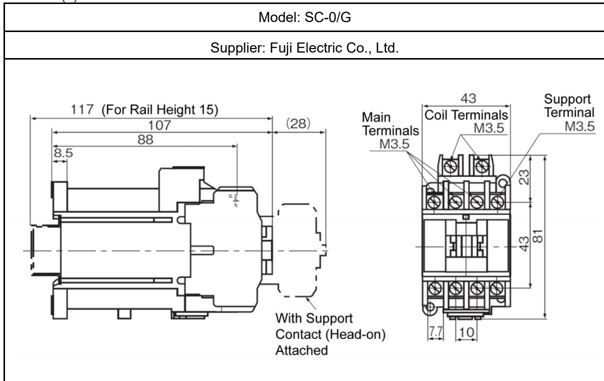
Contactor (1)
