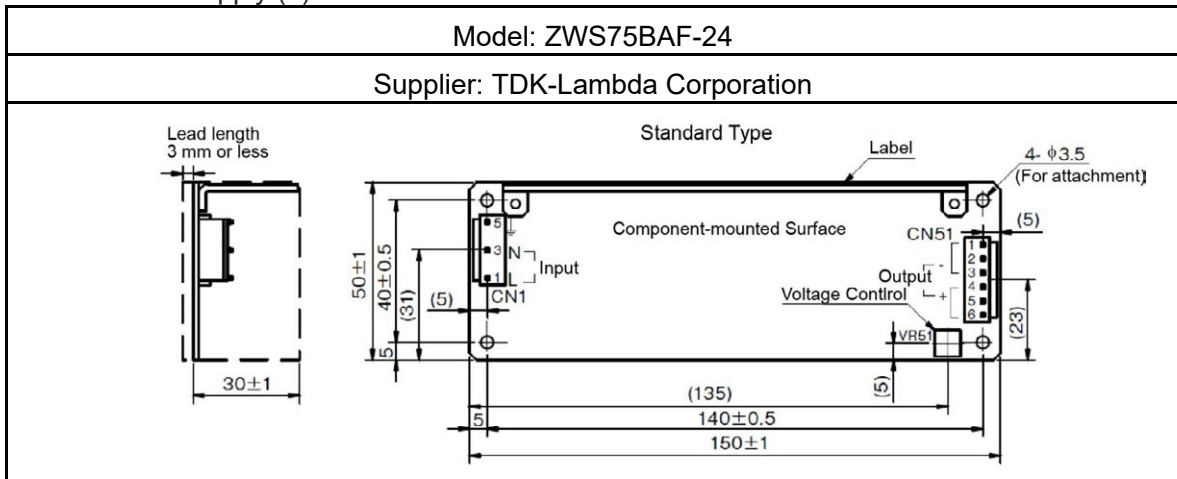
24V DC Power Supply (2)
