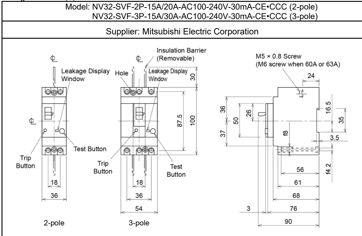
Leakage Breaker (1)
