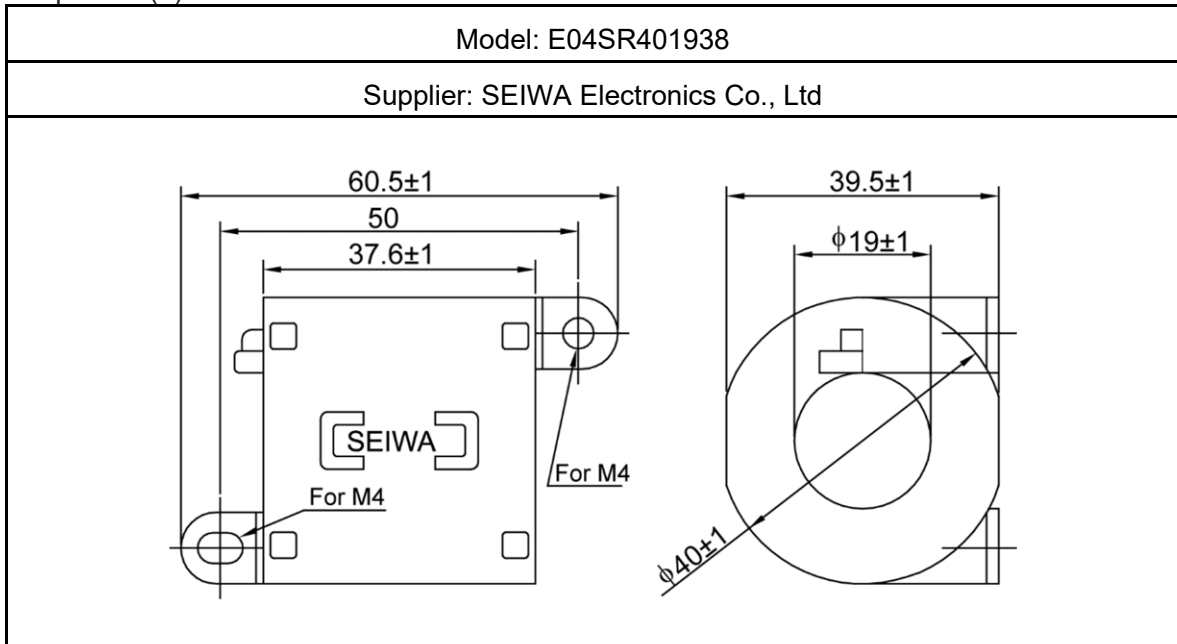
Clamp Filter (2)
