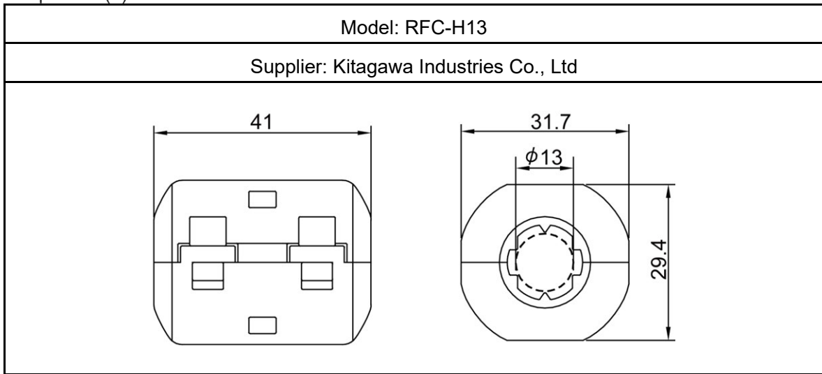
Clamp Filter (3)
