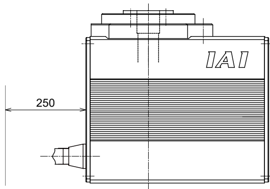
i) RCP2-RTB (Same for other rotary type actuators)
