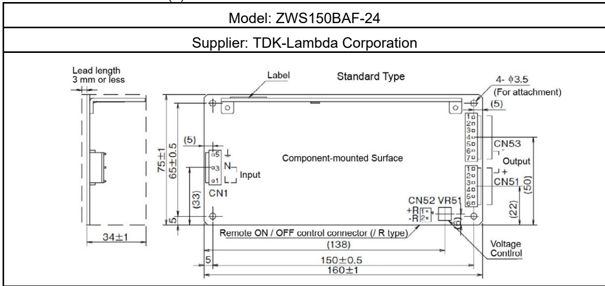
24V DC POWER SUPPLY (1)
