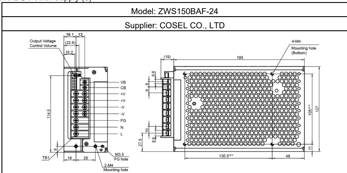
24V DC Power Supply (3)
