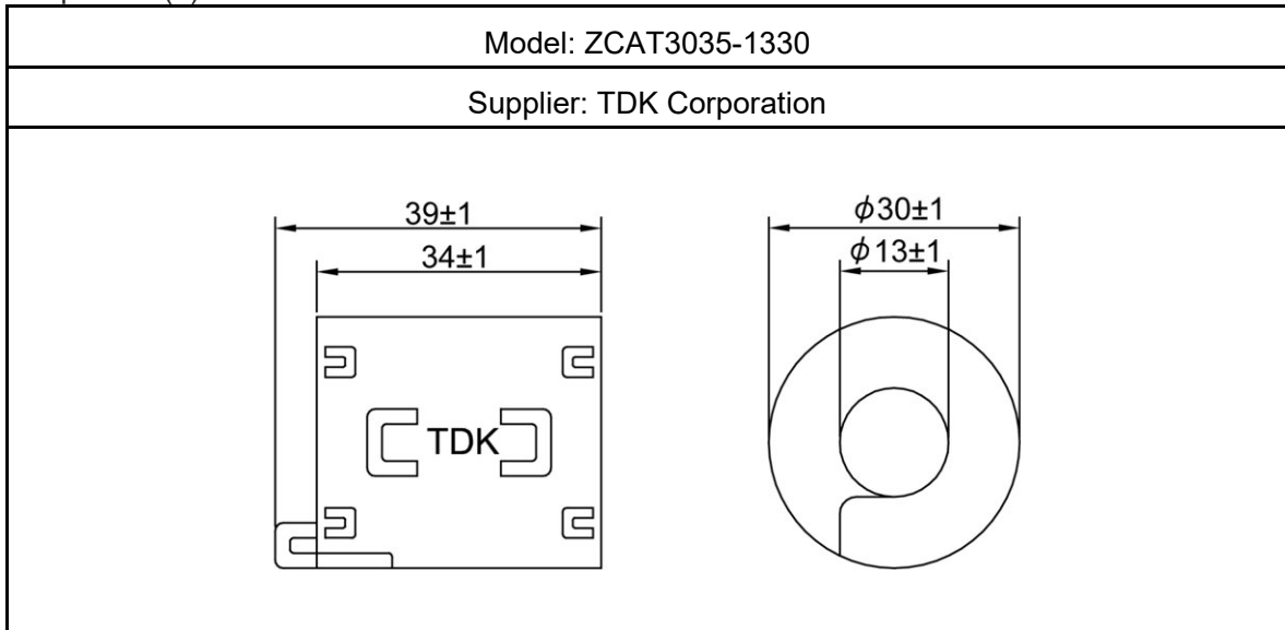
Clamp Filter (1)
