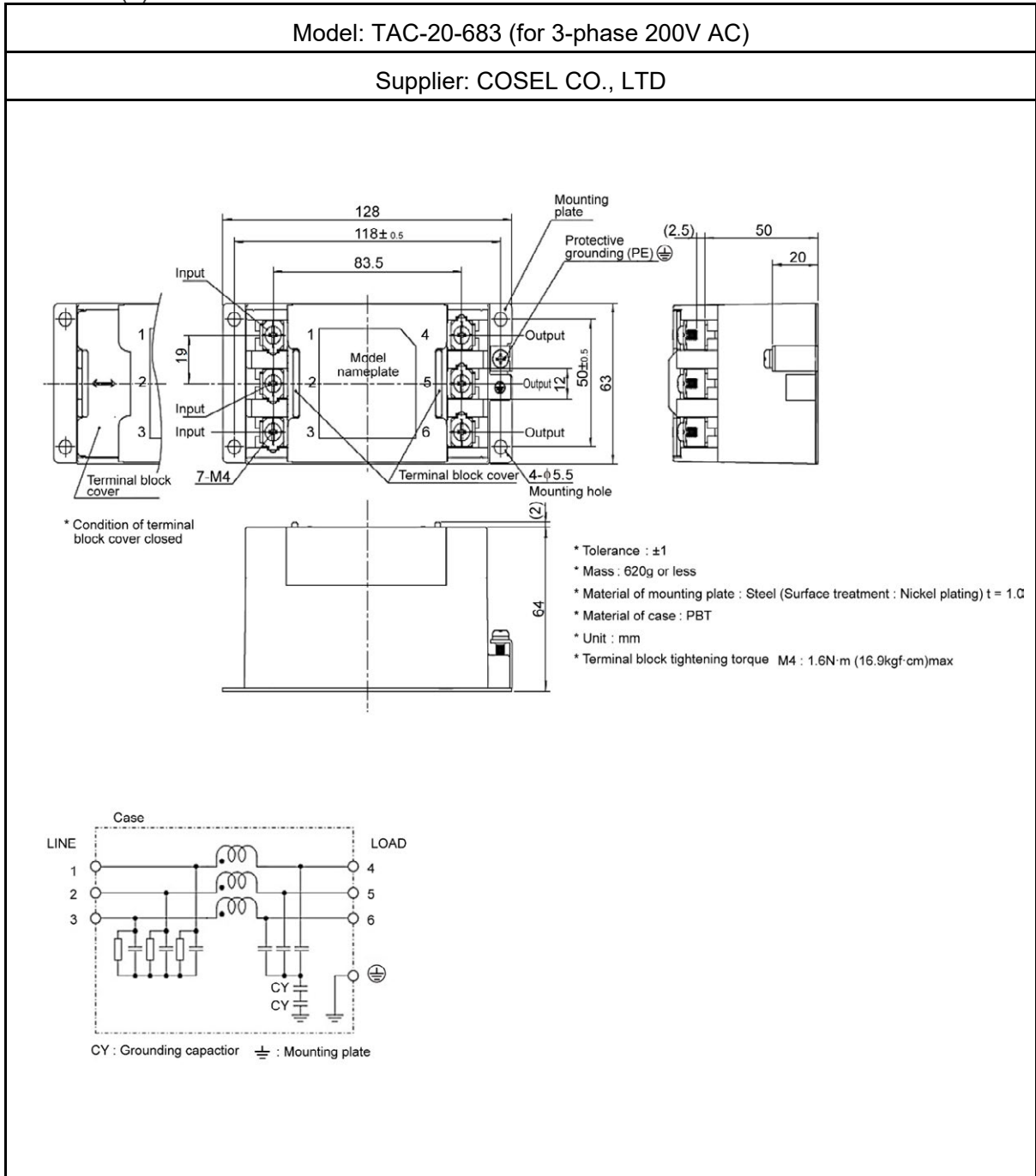
Noise Filter (1)
